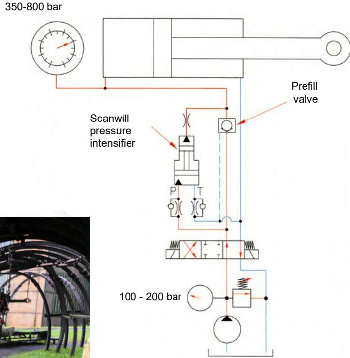
The MP- intensifier (cetop / NG6) for braking circuits
