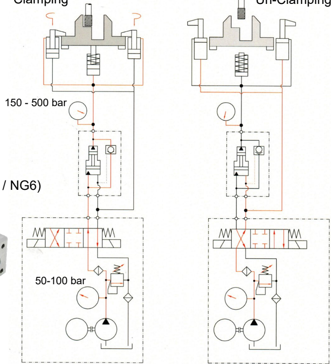
Clamping
