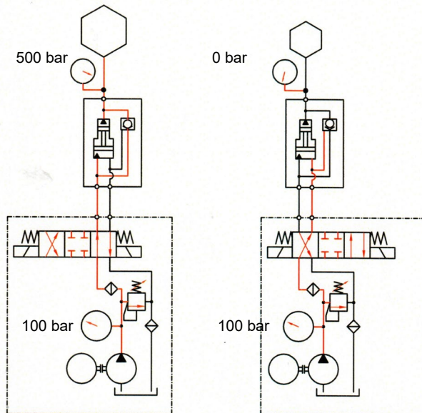
The MP-2000 intensifier (In-Line)
